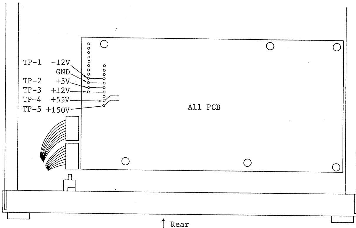
Figure 7-2 (Bottom view)
