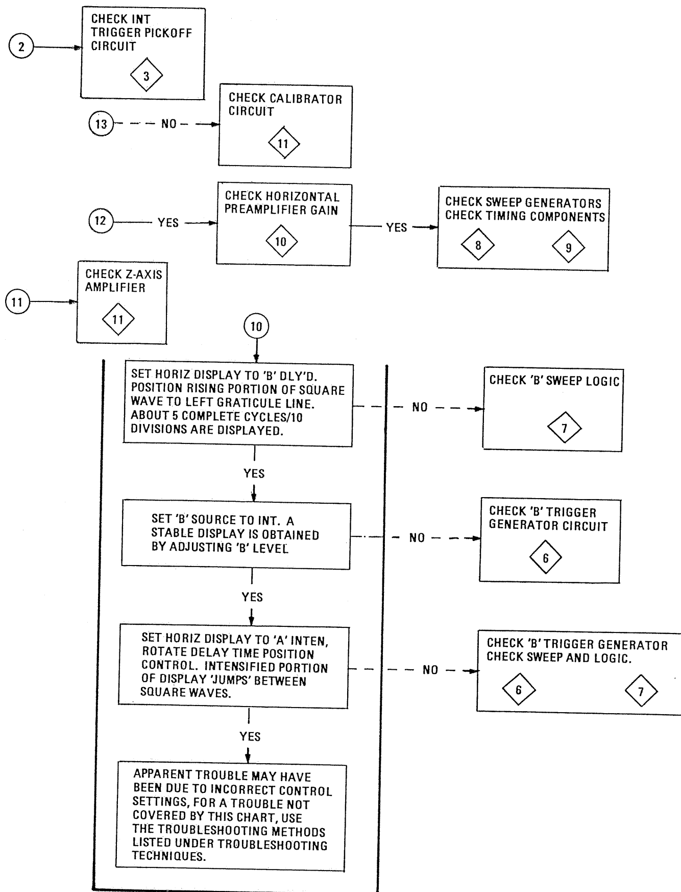
Figure 8-2. TROUBLESHOOTING CHART (SHEET 4 OF 4)
