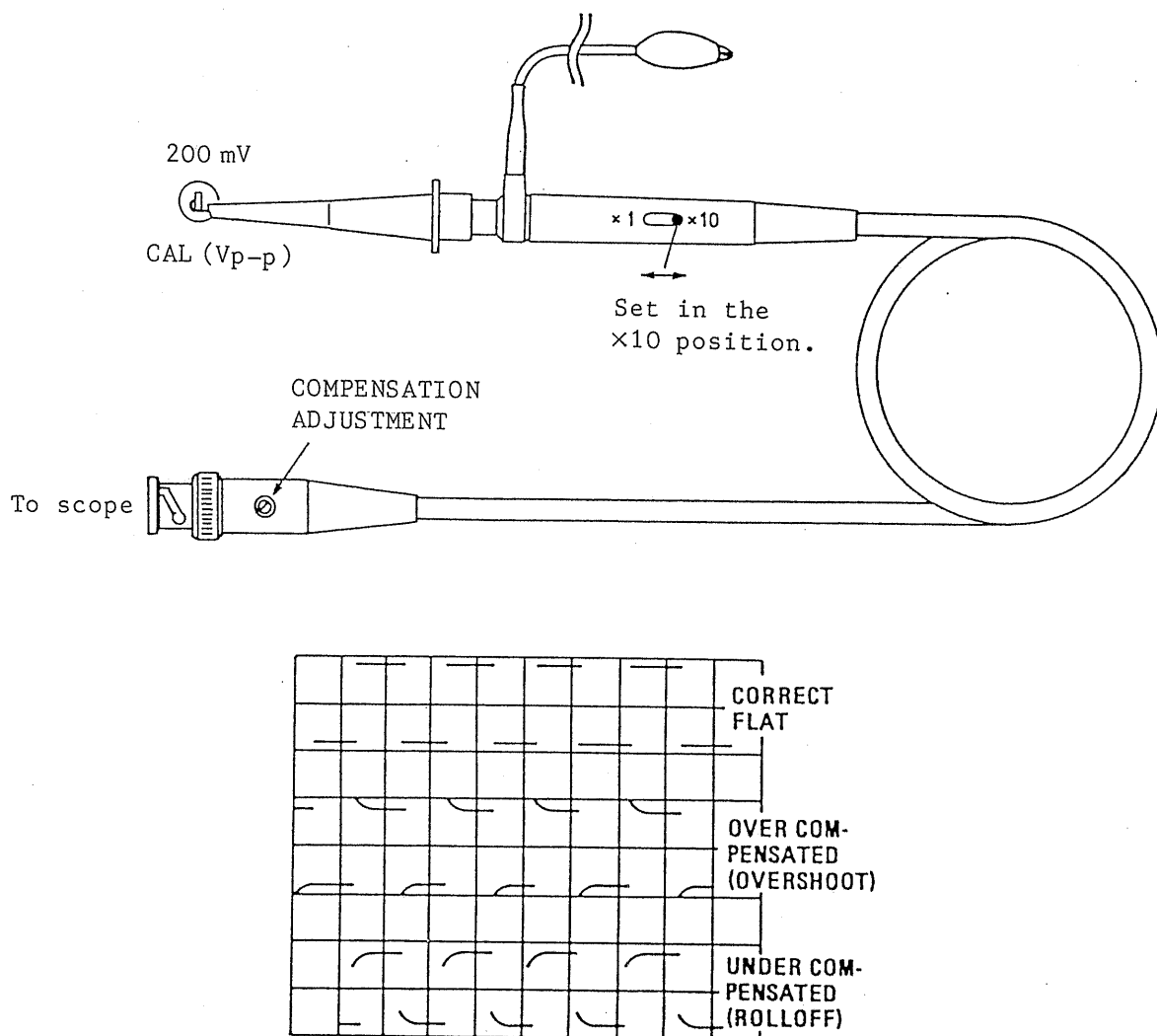
Figure 5-11. PROBE COMPENSATION
