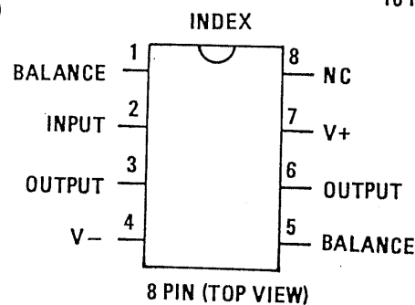
Figure 8-3. SEMICONDUCTOR LEAD CONFIGURATIONS (SHEET 2 OF 2)
